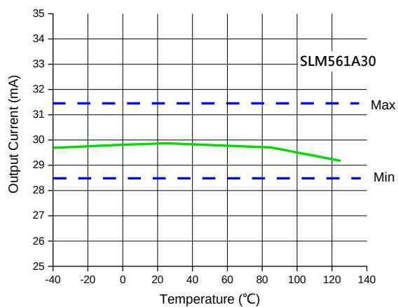
I_P Sink Current Vs Temperature
