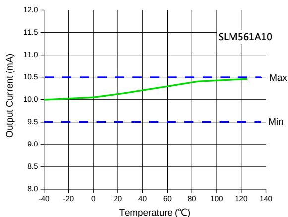
I_P Sink Current Vs Temperature
