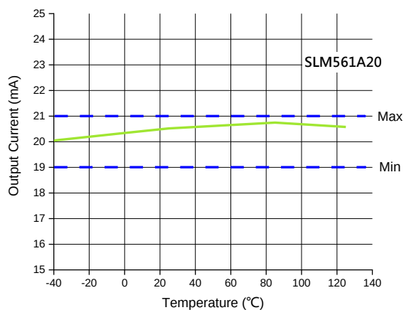
I_P Sink Current Vs Temperature
